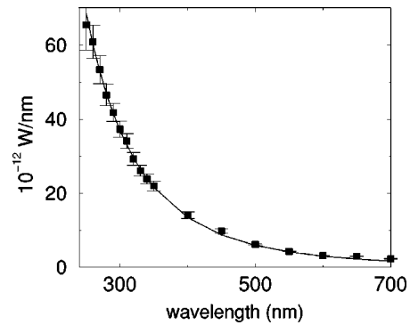
FIG. 5. Spectrum of single-bubble sonoluminescence, for water at 22^\circ\text{C} . The data points are redrawn from Fig. 1 of Hiller et al. (1992). Fits to a blackbody spectrum can be attempted for different temperatures, with best results for about 40 000 K (solid line), higher than the 25 000 K suggested by Hiller et al. (1992).
