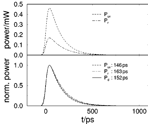
FIG. 44. Theoretically calculated light emission from a R_0 = 5 \mu\text{m} SBSL bubble driven at P_a = 1.3 \text{ atm} and f = 20 \text{ kHz} under the assumption of thermal volume emission. We use T(t) from Fig. 27, and Eq. (68) to evaluate the emission. (a) Absolute power; (b) relative power; line styles as in Fig. 41. The strong dependence of the pulse width on wavelength displayed in that figure is not present here, in agreement with experiments. The total power in the pulse is now much smaller. From Hilgenfeldt et al. (1999b).
