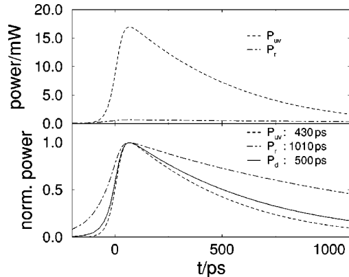
FIG. 41. Theoretically calculated light emission from a R_0 = 5 \mu\text{m} SBSL bubble driven at P_a = 1.3 \text{ atm} and f = 20 \text{ kHz} under the assumption of blackbody radiation, using the temperature dynamics T(t) from Fig. 27 and Eq. (66): dashed lines, pulses in the ultraviolet ( P_{uv} ); dotted lines, pulses in the red ( P_r ) wavelength range; (a) absolute instantaneous powers; (b) pulses normalized to a peak value of 1 for better comparison of their widths; solid line, pulse integrated over the entire range of detectable wavelengths ( P_d ). From Hilgenfeldt et al. (1999b).
