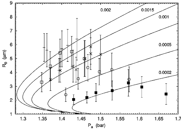
FIG. 34. Experimental data in the phase diagram in the P_a - R_0 plane: +, with an air concentration of c_{\infty}^{\text{air}}/c_0=0.2 ; □, 0.15; ×, 0.1; ■, 0.02. The data lie on the stable diffusive equilibria curves (solid lines) for argon concentrations of c_{\infty}^{\text{Ar}}/c_0=0.002 , 0.0015, 0.001, and 0.0002, confirming the argon rectification theory. Experimental data are taken for as large a P_a as possible, to probe the shape instability threshold. From Simon et al. (2001).
