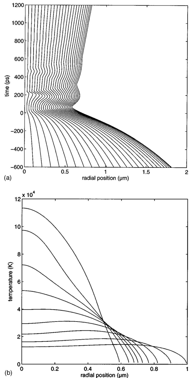
FIG. 16. Motion and temperature in a bubble shortly before collapse: (a) motion history of 20 Lagrangian points inside a R_0 = 4.5 \mu\text{m} bubble driven at P_a = 1.3 \text{ atm} and f = 26.5 \text{ kHz} . Strong wavy motion occurs inside the bubble, but no shock waves develop. (b) Temperature profiles in the bubble for various times around the bubble collapse. The profiles span a time interval of \approx 170 \text{ ps} near the collapse. The temperature at the center increases monotonically, until the maximum temperature is reached at the last snapshot. Note that the temperature profile is smooth, without any discontinuity that would be present with a shock. From Vuong and Szeri (1996).
