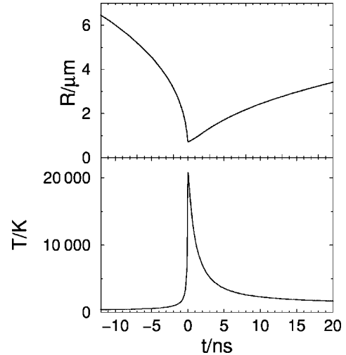
FIG. 27. Temperature inside the SBSL bubble within the simplified model of Hilgenfeldt et al. (1999a, 1999b). (a) Bubble dynamics and (b) temperature dynamics of R_0 = 5 \mu\text{m} bubble driven at 1.3-atm pressure amplitude at f = 20 \text{ kHz} . The temperature is calculated via Eq. (38); the full width at half maximum of the asymmetric peak is \approx 1 \text{ ns} .
