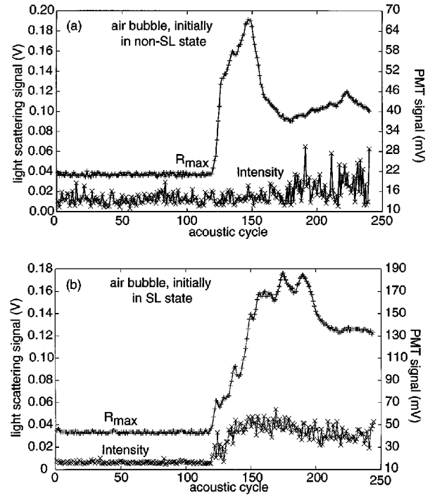
FIG. 32. (+) The maximum radius and (x) sonoluminescence intensity of an air bubble plotted over approximately 240 consecutive cycles. The “radius” is actually a signal level, proportional to the square of maximum radius (assuming a geometrical optics limit for Mie scattering from a sphere). (a) The bubble is initially below the light-emission threshold (the photomultiplier tube signal level corresponds to noise). At approximately the 120th acoustic cycle, the drive pressure is rapidly increased to a value above the SBSL threshold. (b) For this case, the bubble is initially in a stable sonoluminescing state. The drive pressure is then rapidly reduced to a value below the light-emission threshold, and then quickly increased again after a time period of approximately 90 ms. In both (a) and (b), the drive amplitudes at the lower and upper values are the same. From Matula and Crum (1998).
