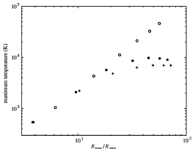
FIG. 26. Dependence of the bubble center temperature on the compression ratio R_{\max}/R_{\min} . \circ , calculations without water vapor; * , with water vapor, but no reactions; + , with water vapor, including reactions. Note the logarithmic scale on the axes. From Storey and Szeri (2000).
