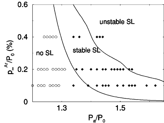
FIG. 9. Phase diagram in the p_{\infty}^{\text{Ar}}/P_0 vs P_a/P_0 parameter space, according to the hydrodynamic/chemical theory of Hilgenfeldt et al. (1996) and Lohse et al. (1997). The driving frequency is f=33.4 kHz. The three phases represent stable SL, unstable SL, and no SL. The symbols represent measurements by Ketterling and Apfel (1998), either stable sonoluminescing bubbles ( \blacklozenge ) or stable, nonsonoluminescing bubbles ( \circ ), showing good agreement with the earlier theoretical predictions.
