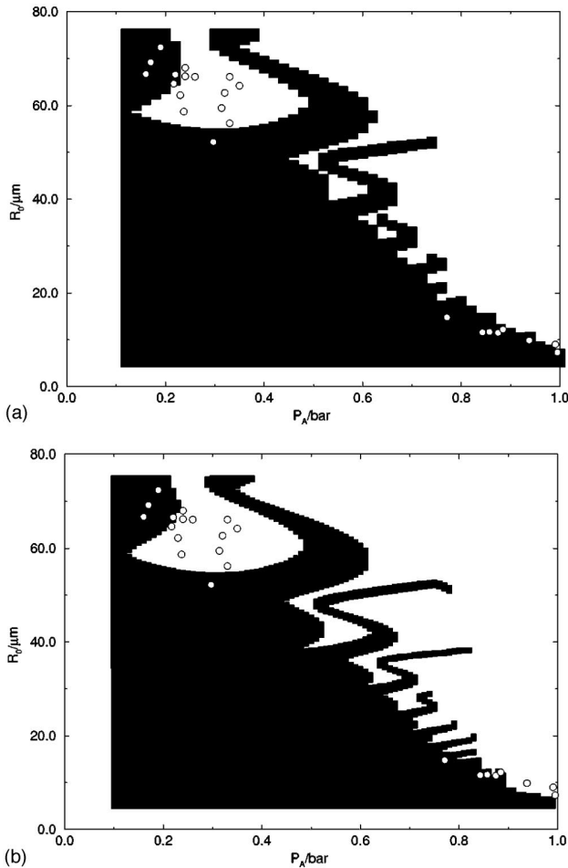
FIG. 35. Comparison of boundary layer approximation and full integrodifferential equation: (a) The dark area is the calculated stability region for the n=2 mode for an air bubble in water at f=20.6 kHz. The open circles are the data of Holt and Gaitan (1996; Gaitan and Holt, 1999). The calculation employed the boundary layer approximation. (b) Same calculation as above, but based on the full integrodifferential equations, rather than the boundary layer approximation: Hardly any difference as compared to (a) can be observed. From Hao and Prosperetti (1999).
