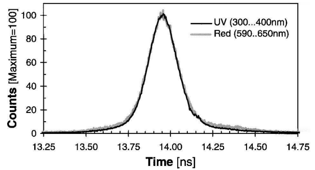
FIG. 13. First measurement of SBSL pulse widths. The parameters were P_d=1.2 bars, f=20 kHz, and the gas concentration was 1.8-mg/l O_2 . Both the width in the red and the ultraviolet spectral range were measured. The indistinguishable widths rule out blackbody radiation, but not a thermal emission process in general. From Gompf et al. (1997).
