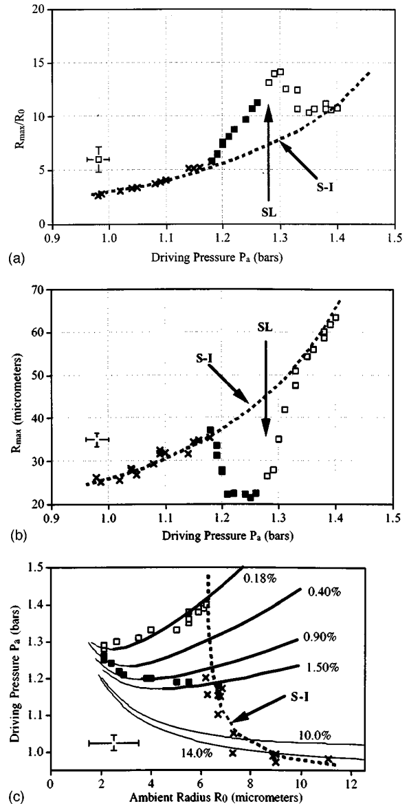
FIG. 33. Experimental maximal bubble radius and phase diagram for SBSL: (a) the ratio between maximum radius R_{\text{max}} and ambient radius R_0 ; (b) R_{\text{max}} as a function of the driving pressure P_a ; (c) data points in the P_a vs R_0 phase space; \square , stable glowing bubbles; \blacksquare , stable nonglowing bubbles; + , unstable, nonglowing bubbles; dashed line, the experimentally found shape instability; solid lines, theoretical diffusive equilibria for various argon concentrations. To compare this figure with theoretical phase diagrams such as Fig. 10 or other experimental results such as Fig. 12, one should exchange abscissa and ordinate. From Gaitan and Holt (1999).
