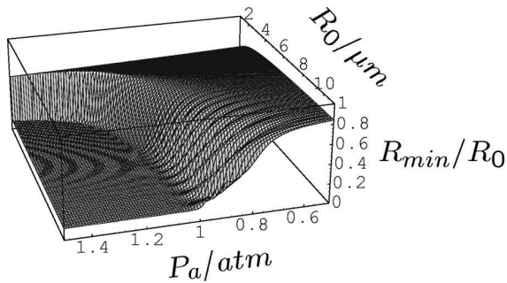
FIG. 29. Minimal bubble radius R_{\min}/R_0 as a function of R_0 and P_a . The frequency is f=26.5 kHz.
